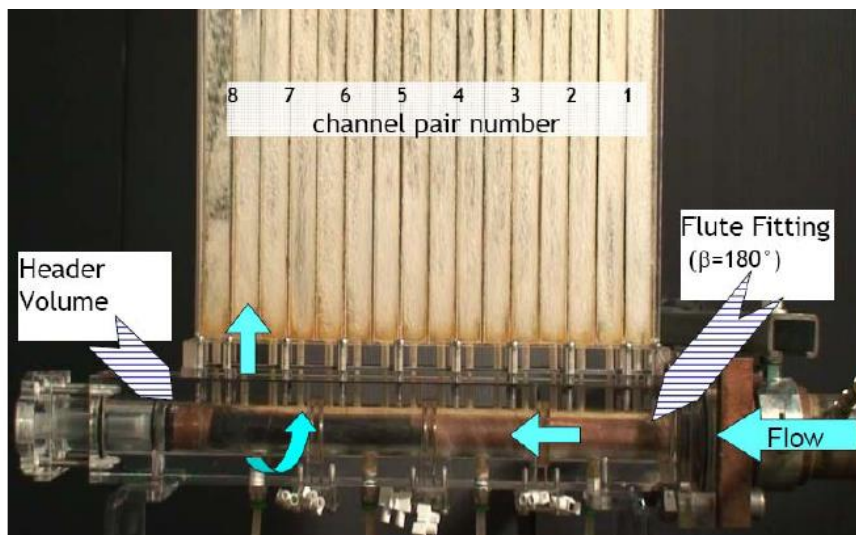
Figure 1. Test Section
