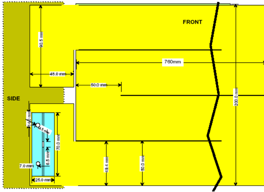
Fig. 1. Heater geometry and related connector for electrical supply.
